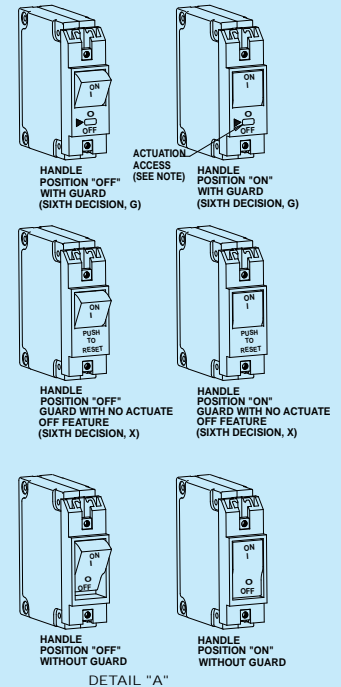
DETAIL "A"
